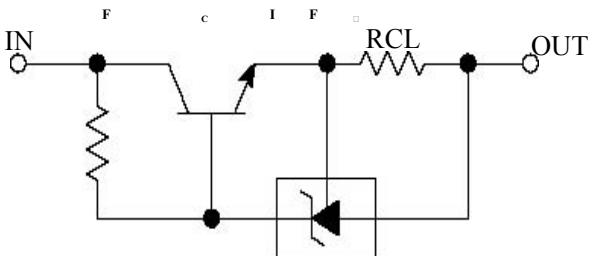
Constant Current Source
