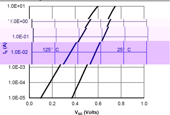
Figure 6: Body-Diode Characteristics
