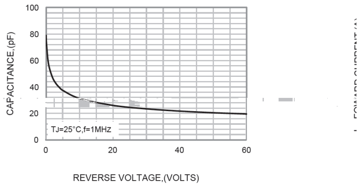
FIG.3-TYPICAL JUNCTION CAPACITANCE
