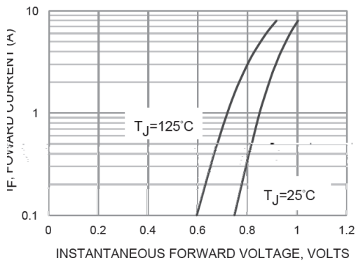
FIG.4-TYPICAL FORWARD CHARACTERISTICS
