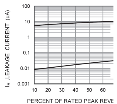
FIG.5-TYPICAL REVERSE CHARACTERISTICS
